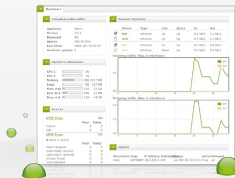
Endian Dashboard
